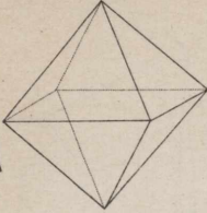
2. Octaeder.
