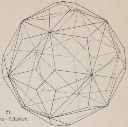
Pyramiden-Trioctaeder.
