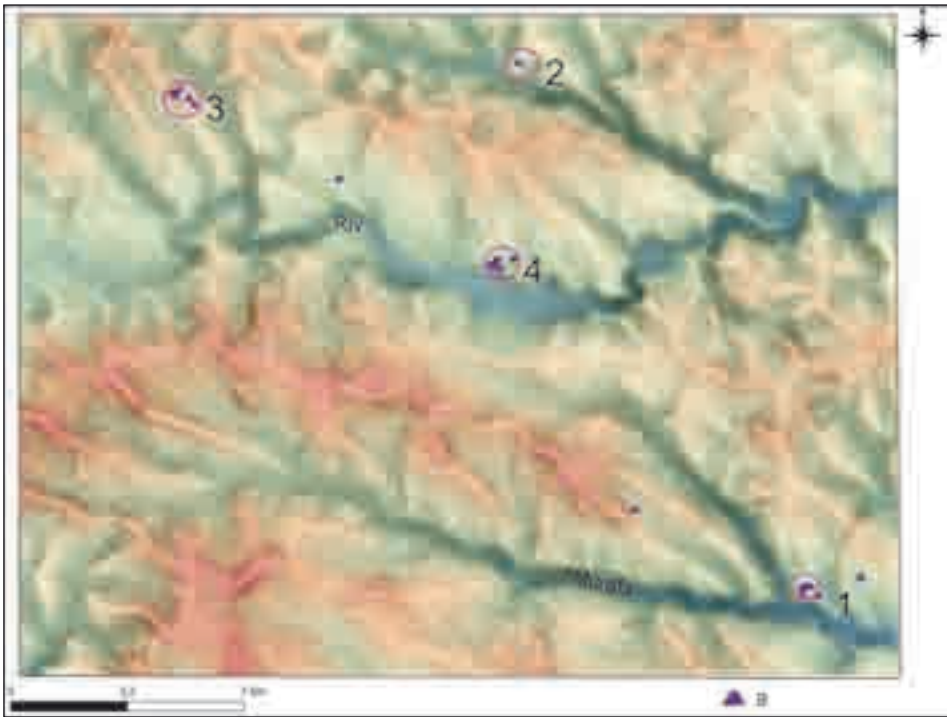
Fig. 2. Location of barrows in the study area. Prepared by M. Ławniczak
