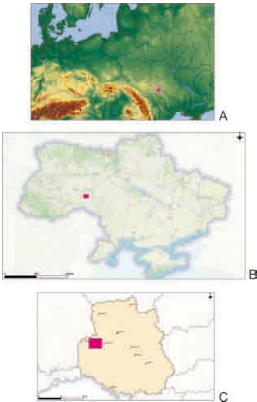
Fig. 1. Location of the study area: A – in the European context; B – in Ukraine; C – in Vinnytsia oblast . Prepared by M. Ławniczak and M. Szmyt
