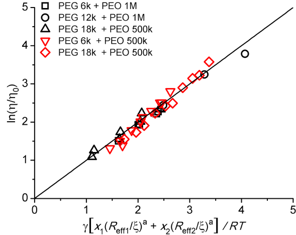
Figure 4: Results of fluorescence correlation spectroscopy measurements for double-entangled aqueous PEG/PEO solution mixtures. Diffusion of two probes – rhodamine 110 (black symbols) and apotransferrin labeled with Atto 488 (red symbols) – was observed. A range of concentrations up to 40% (w/w) for PEGs and up to 2.5% for PEOs is covered (see Supporting Information for a full sample and data table). Data are plotted in terms of relative, effective viscosity experienced by the probes according to Equation 14, which corresponds to the solid line. No parameters were fitted; the applied values of both \gamma and a were independently established in solutions containing a single polymer species (see Figure 3 and Ref. 24, respectively).
