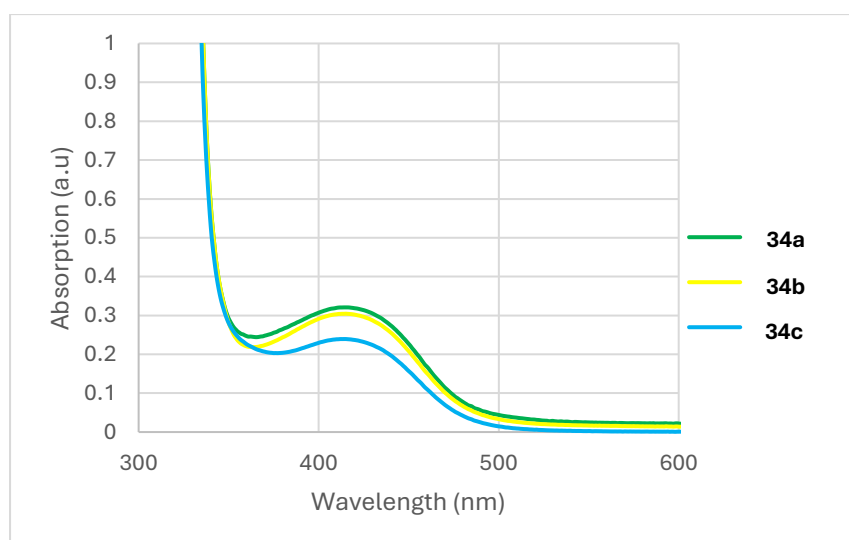
Figure S7: UV-Vis spectra of 4-diazo-2H-benzo[e][1,2]thiazin-3(4H)-one 1,1-dioxides. c = 0.006 \text{ M (DCM)}
