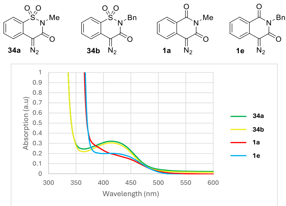
Figure S8: Comparing the UV-Vis spectra of the two families of diazo compound. c = 0.006 \text{ M} (DCM)
