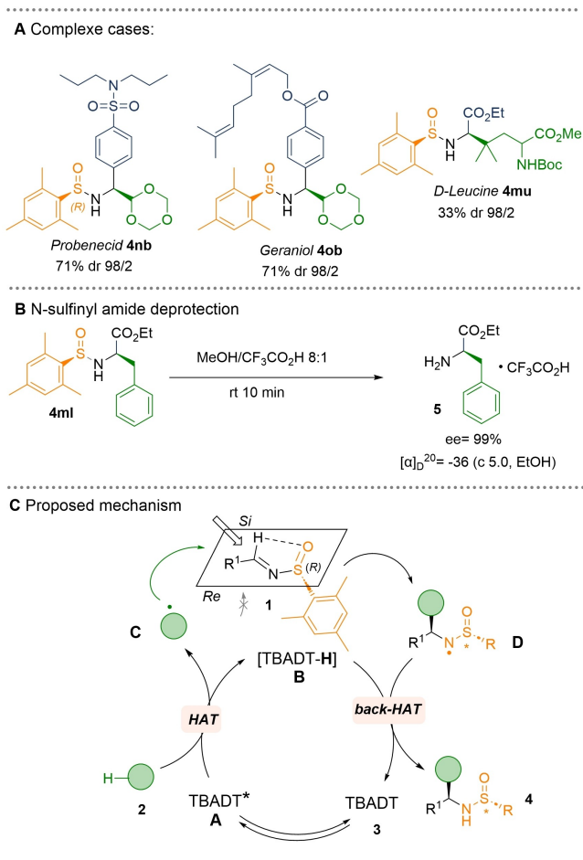
Scheme 5. (A) Functionalization of complex molecules (B) Chiral auxiliary cleavage and determination of the absolute configuration of 5. (C) Proposed mechanism for the photocatalyzed HAT transformation.
