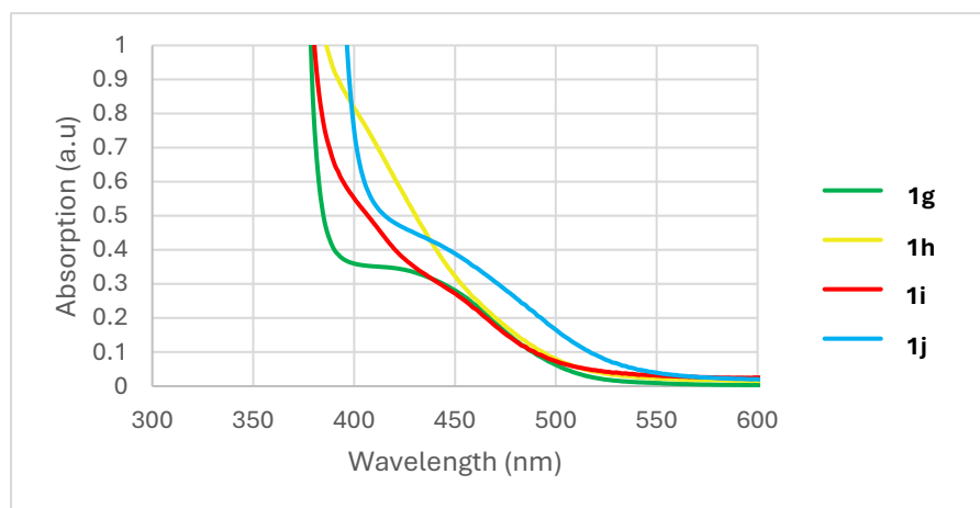
Figure S6: Influence of different functional groups at the 7-position on the UV-Vis spectra. c = 0.006 \text{ M (DCM)}
