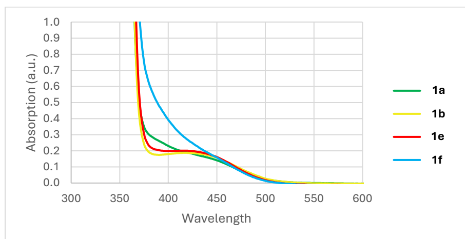
Figure S4: Influence of N -substituents on UV-Vis spectra. c = 0.006 M (DCM).
