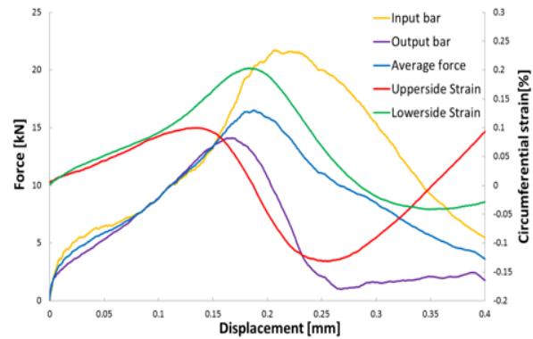
Fig. 2. Force and circumferential strain vs displacement obtained by the SHPB technique
