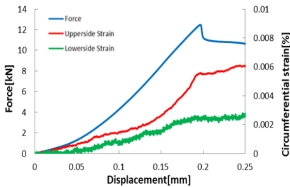
Fig. 1. Force and circumferential strain vs displacement obtained by the quasi-static test
