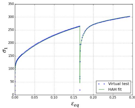
Figure 2: Modeling of the Bauschinger effect for the aluminium alloy AA5182.
